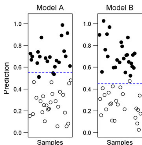
Fig. 7 Difference between ranking and classification. The two scatter plots show the predicted class probabilities for 50 new samples by two biomarker models. Both models are able to rank all new samples correctly. Therefore, they both will have the same AUC (1.0) but exhibit different error rates (3/50 and 1/50 respectively) due to their different decision boundaries, which were determined during the model creation process
